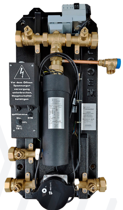
HYDRAULIKSTATION 20
